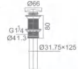
B006-2 Pop-up waste (Antique brass) 1 1/4 全牙大盖弹跳 (红古铜)
