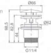
B099-1 Pop up Waste (Plastic+Brass+SUS304) 銅塑料彈跳去水 (G1-1/4)
