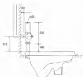
Flush with pedal Automatic induction toilet (all copper) AR-9011A (Direct current)
