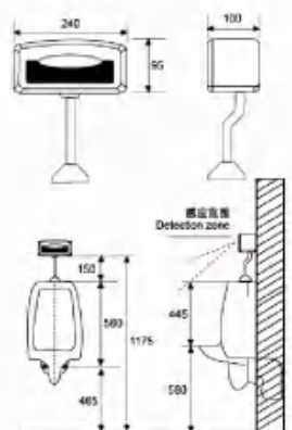
Surface mounted urinal sensor flusher AR-8011A (Direct current) AR-8011AB (AC and DC)
