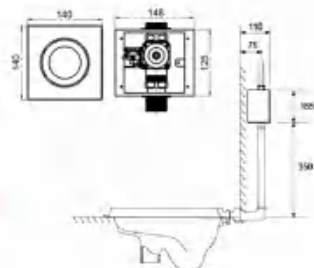
Electronic flushing with touch Automatic induction toilet AR-9016A (Direct current) AR-9016B (Communicate)
