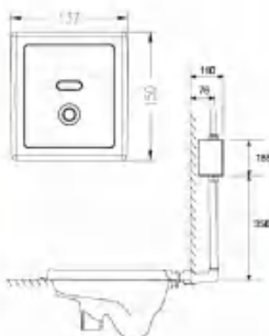
With mechanical manual flushing Automatic induction toilet AR-9003A (Direct current) AR-9003B (Communicate)
