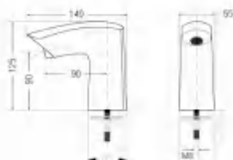
Automatic sensor faucet (Mouth sensation)
