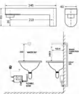
Automatic sensor faucet AR-6H49A (Direct current) AR-6H49AB (AC and DC)
