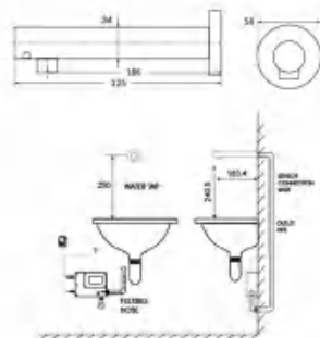
Automatic sensor faucet AR-6186A (Direct current) AR-6186AB (AC and DC)
