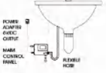
Automatic sensor faucet AR-6165A (Direct current) AR-6165AB (AC and DC)
