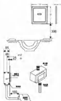
Automatic induction toilet AR-9001A (Direct current) AR-9001B (Communicate)
