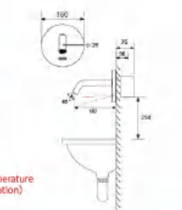
Semi-automatic (Temperature regulation) sensor faucet AR-6270-1A (Direct current) AR-6270-1AB (AC and DC)
