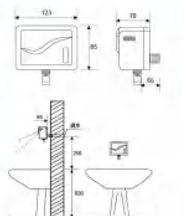
Wave the water to the boil, then wave it off Semi-automatic induction hand washing machine AR-6268A (Direct current) AR-6268AB (AC and DC)
