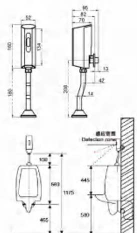
Surface mounted urinal sensor flusher AR-8018A (Direct current)
