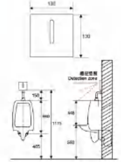
Urinal sensor flushing device (concealed) AR-8006A (Direct current) AR-8006AB (Communicate)
