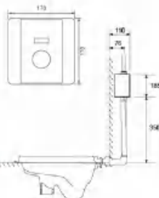
Electronic flushing with touch Automatic induction toilet AR-9015A (Direct current) AR-9015B (Communicate)
