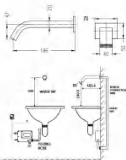
Automatic sensor faucet AR-6116A (Direct current) AR-6116AB (AC and DC)
