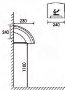
Automatic induction hand dryer (1800W) AR-3001B (Communicate)
