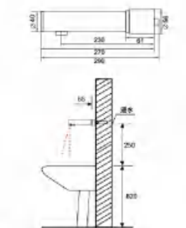
Automatic sensor faucet (Integrated) AR-6888-1A (Direct current) AR-6888-1AB (AC and DC)
