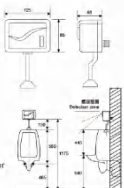
Surface mounted urinal sensor flusher AR-8012A (Direct current) AR-8012AB (AC and DC)
