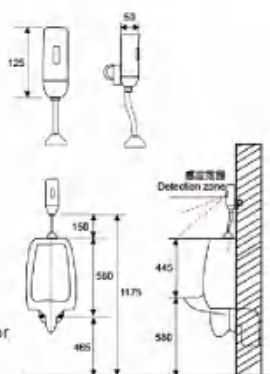
Surface mounted urinal sensor flusher (all copper) AR-8010A (Direct current)
