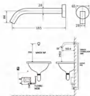
Automatic sensor faucet AR-6113A (Direct current) AR-6113AB (AC and DC)
