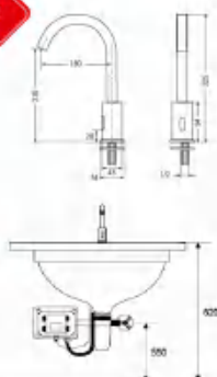
Semi-automatic sensor faucet
