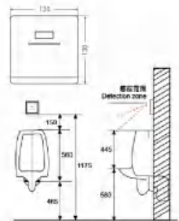
Urinal sensor flushing device (concealed) AR-8909B (Communicate) With LED light
