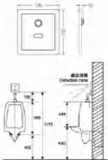
Urinal sensor flushing device (concealed) AR-8005A (Direct current) AR-8005B (Communicate)
