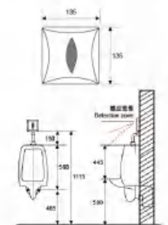
Urinal sensor flushing device (concealed) AR-8004A (Direct current) AR-8004AB (Communicate)
