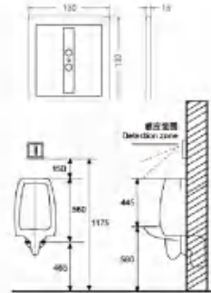
Urinal sensor flushing device (concealed) AR-8003A (Direct current) AR-8003B (Communicate)
