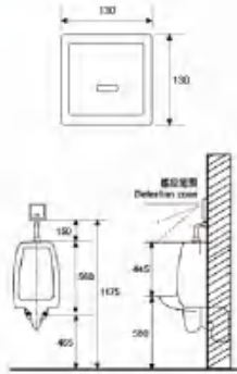
Urinal sensor flushing device (concealed) AR-8001-1A (Direct current) AR-8001-1AB (Communicate)
