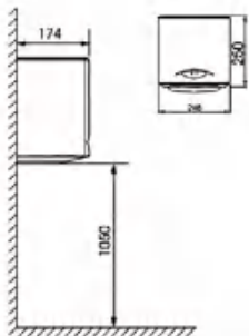
Automatic induction hand dryer (high speed) AR-3003B (Communicate)
