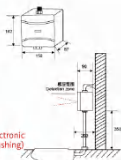
Surface mounted sensor flush toilet AR-9010A (Direct current) AR-9010B (Communicate)
