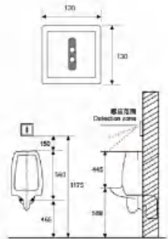
Urinal sensor flushing device (concealed) AR-8002A (Direct current) AR-8002AB (Communicate)
